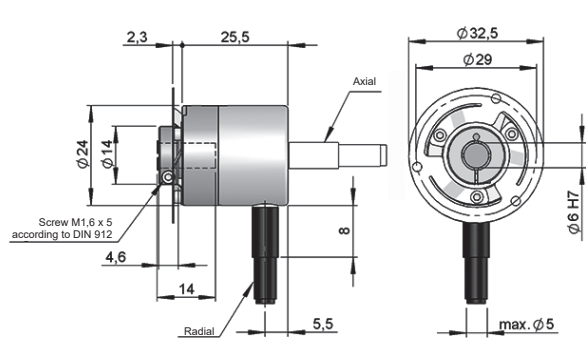
Drawing blind hollow shaft mechanical option type 3, connection type 1/2
